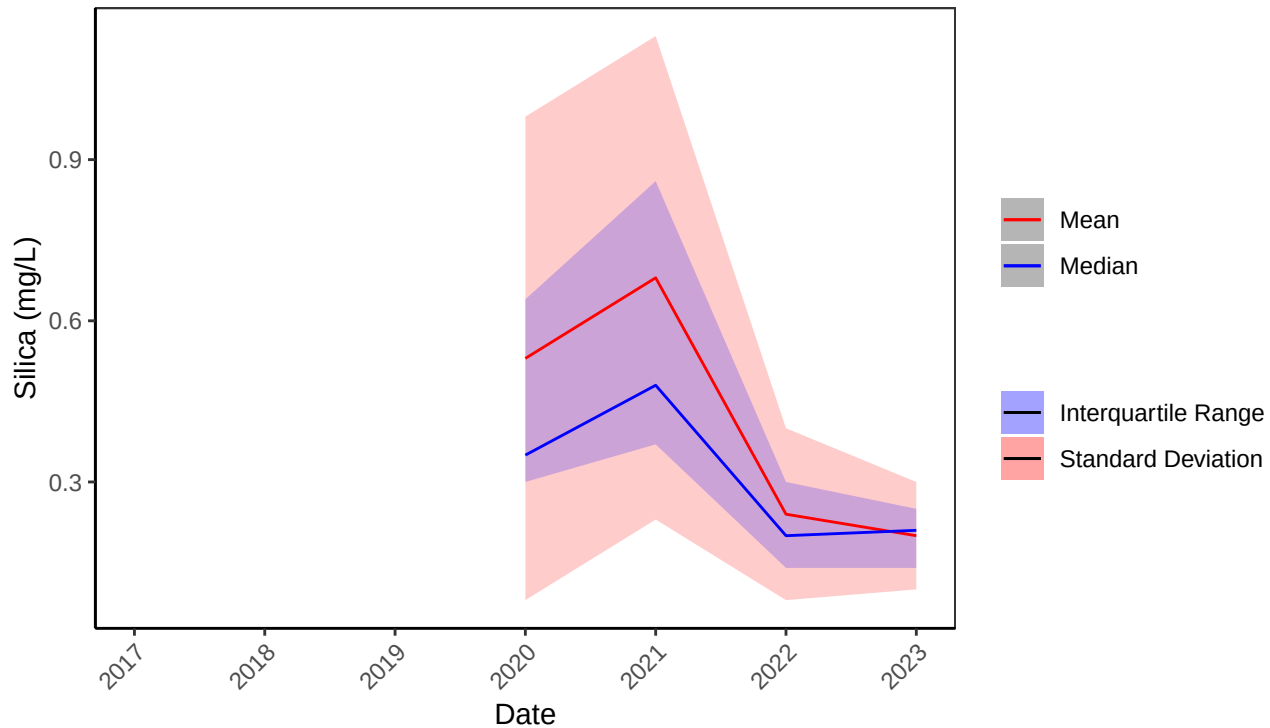
B2 Raceway 1 Silica (mg/L) Yearly Statistics
